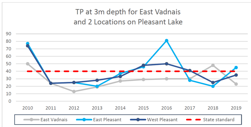
Figure 32: Total Phosphorus Comparison between East Vadnais Lake and Pleasant Lake
