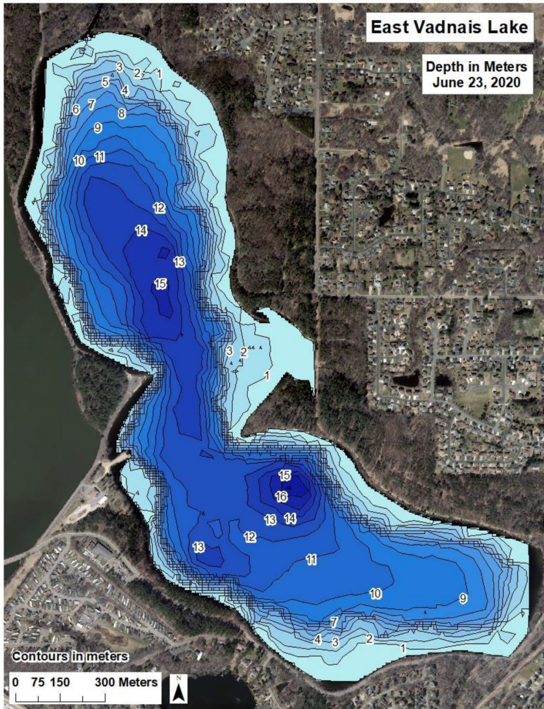
Figure 5. East Vadnais Lake depth with one-meter contours – June 2020 map used.
