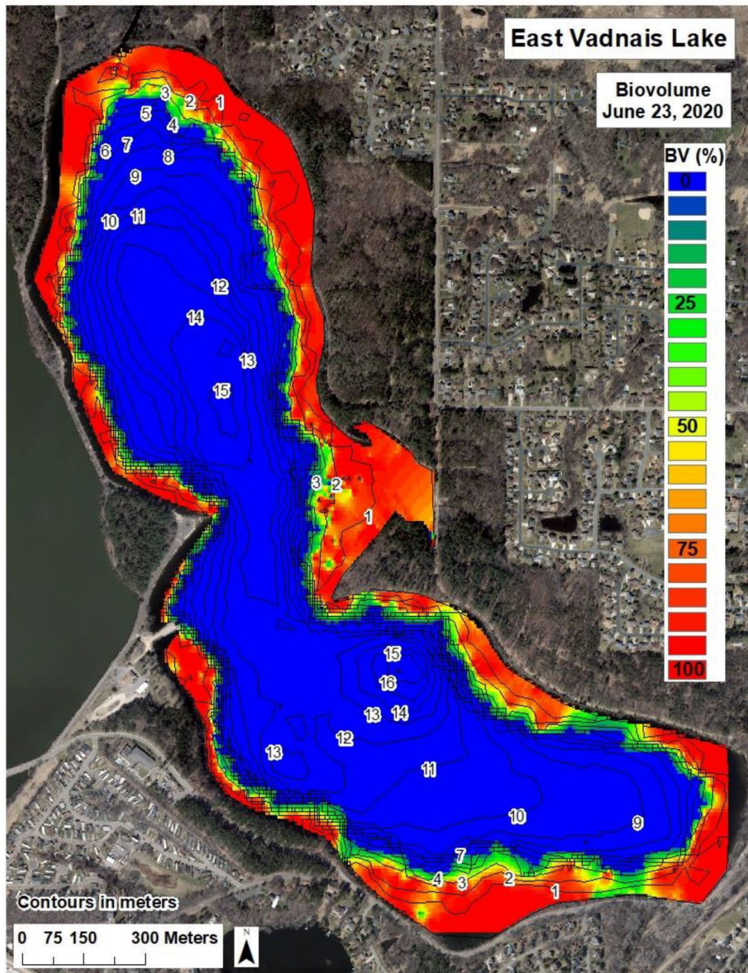
Figure 6. East Vadnais Lake vegetation biovolume with one-meter contours. Percent values range from zero to one hundred; Blue = 0%, Yellow = 50% and Red = 100%.
