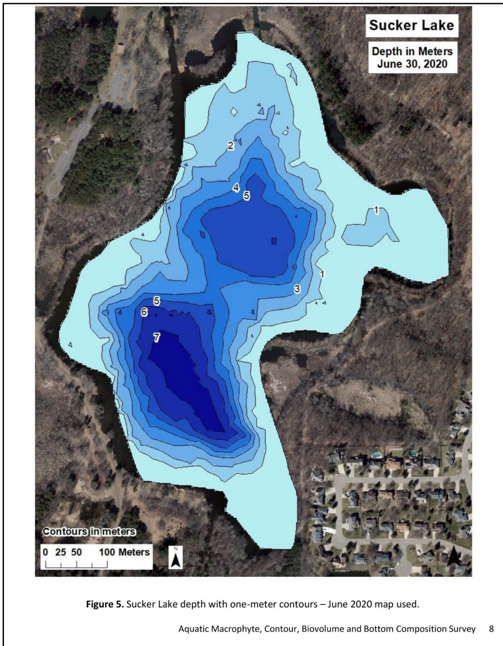
Figure 18: Sucker Lake Depths with 1-meter Contours
